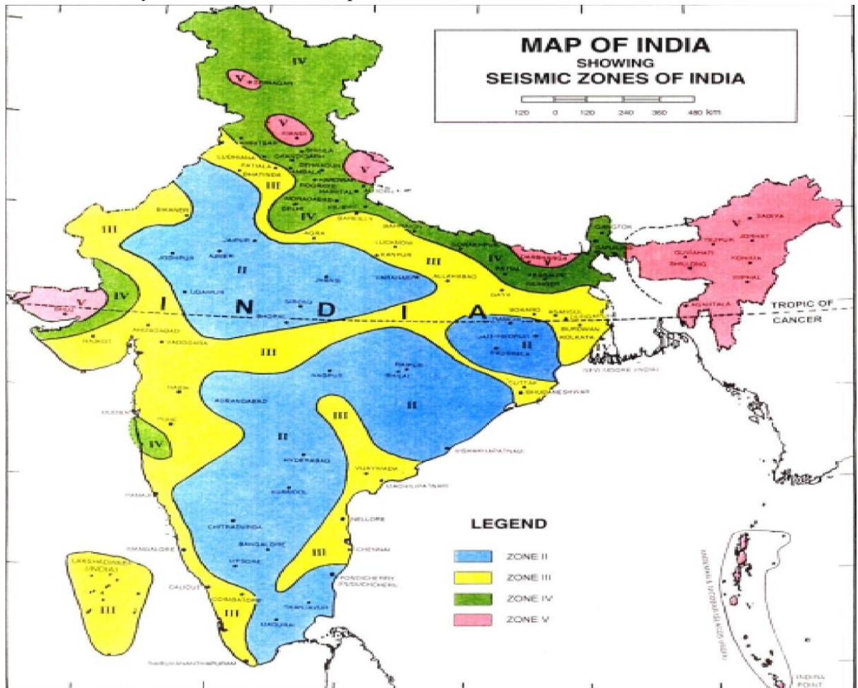
Figure: Seismic Zone Map of India as Per IS: 1893 Part 1-2002
