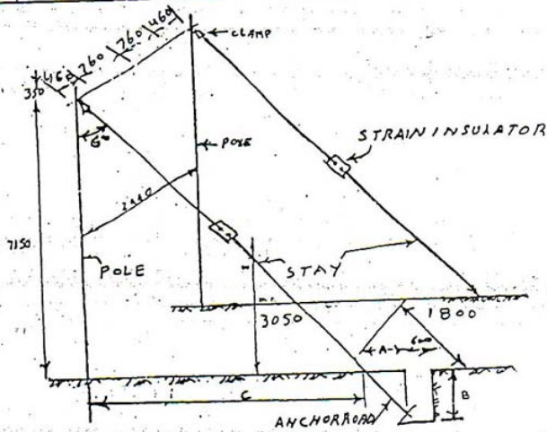
DISTANCES FOR 30° AND 45° ANGLES OF STAY WIRE WITH POLE
