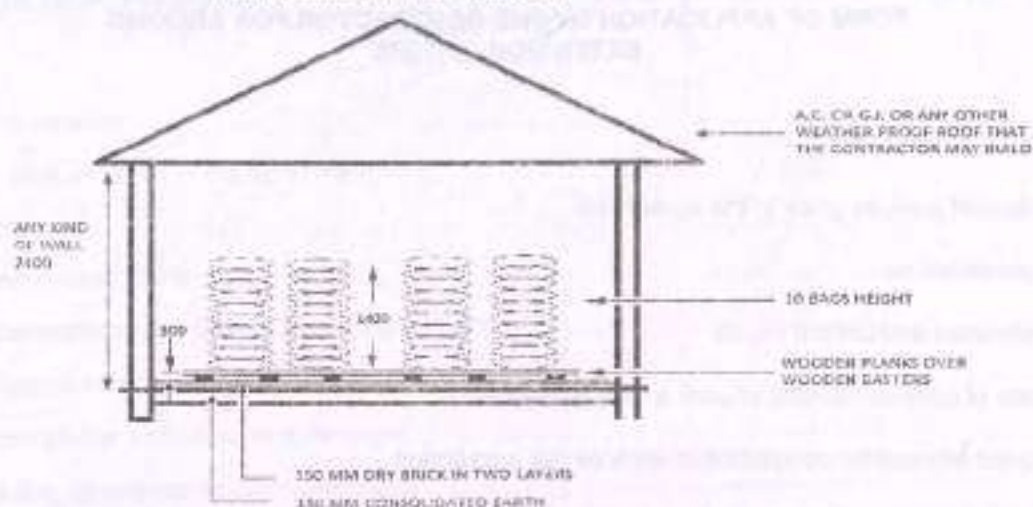
SKETCH OF CEMENT GODOWN
