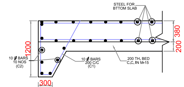
REINFORCEMENT DETAILS OF R.C.C.CUT-OFF AT SECTION 1-1
