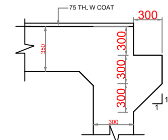
DETAILS AT-P
