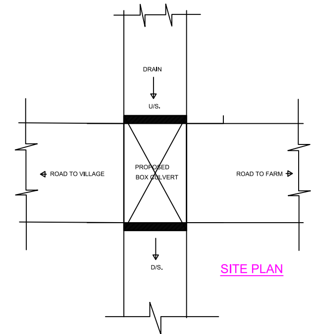
DETAILS AT-P
