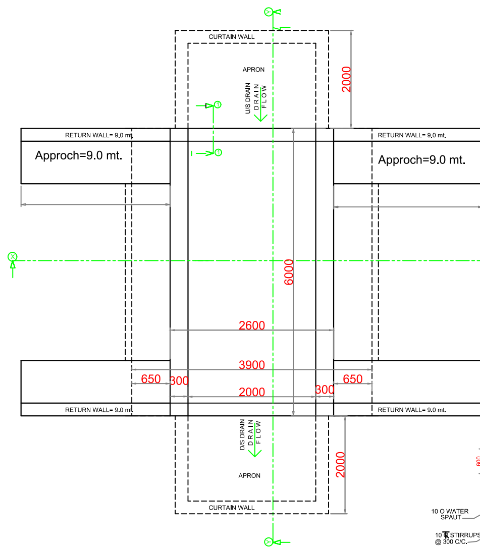
PLAN
