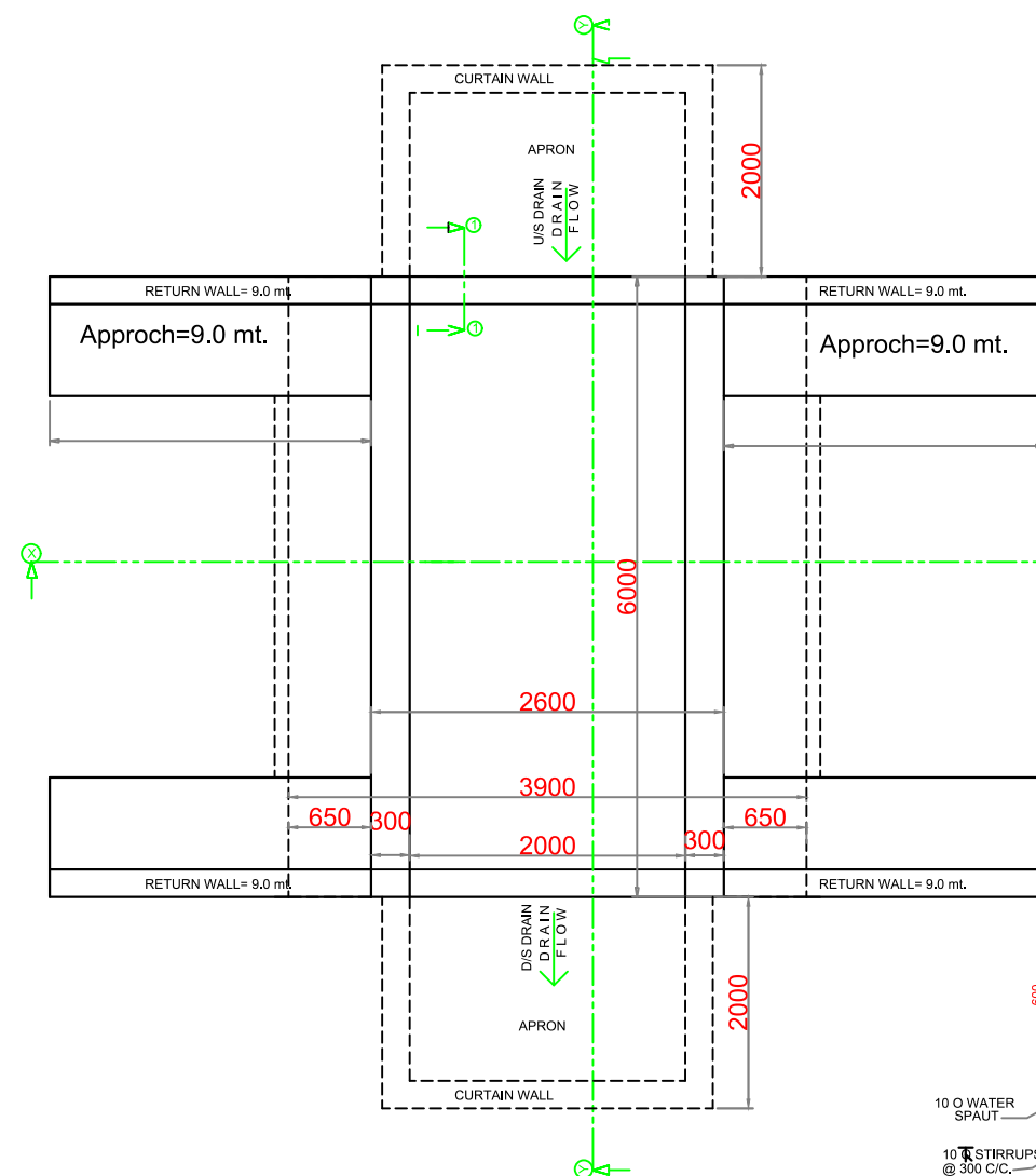
PLAN
