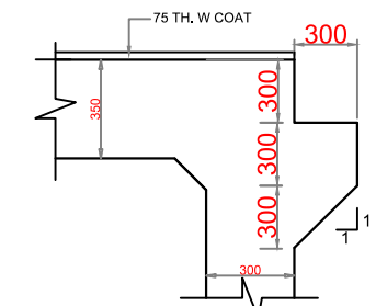
DETAILS AT-P
