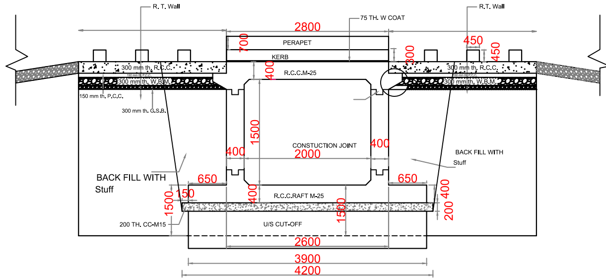
SECTIONAL ELEVATION :~ 'X-X'
