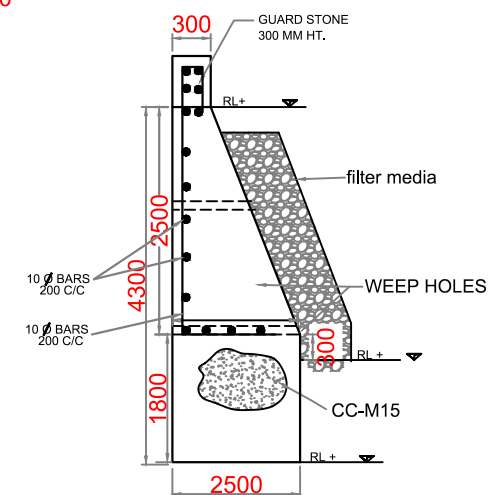
RETURN WALL SECTION C-C
