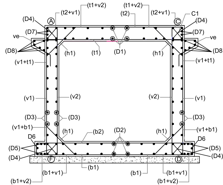
REINFORCEMENT DETAILS OF R.C.C. BOX
