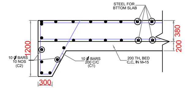
REINFORCEMENT DETAILS OF R.C.C.CUT-OFF AT SECTION 1-1
