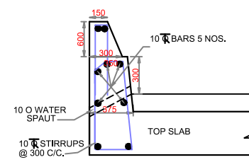
REINFORCEMENT DETAILS OF KERB & GUARD WALL ( Section a-a )
