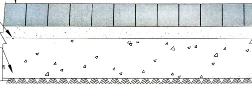
TYPICAL CROSS SECTION OF 60 mm BLOCK PAVEMENT USE IN FOOTPATH
