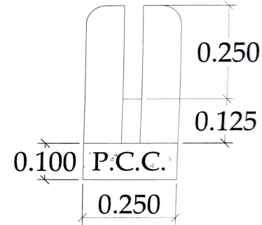
DIMENSIONS OF KERB STONE IN METERS
