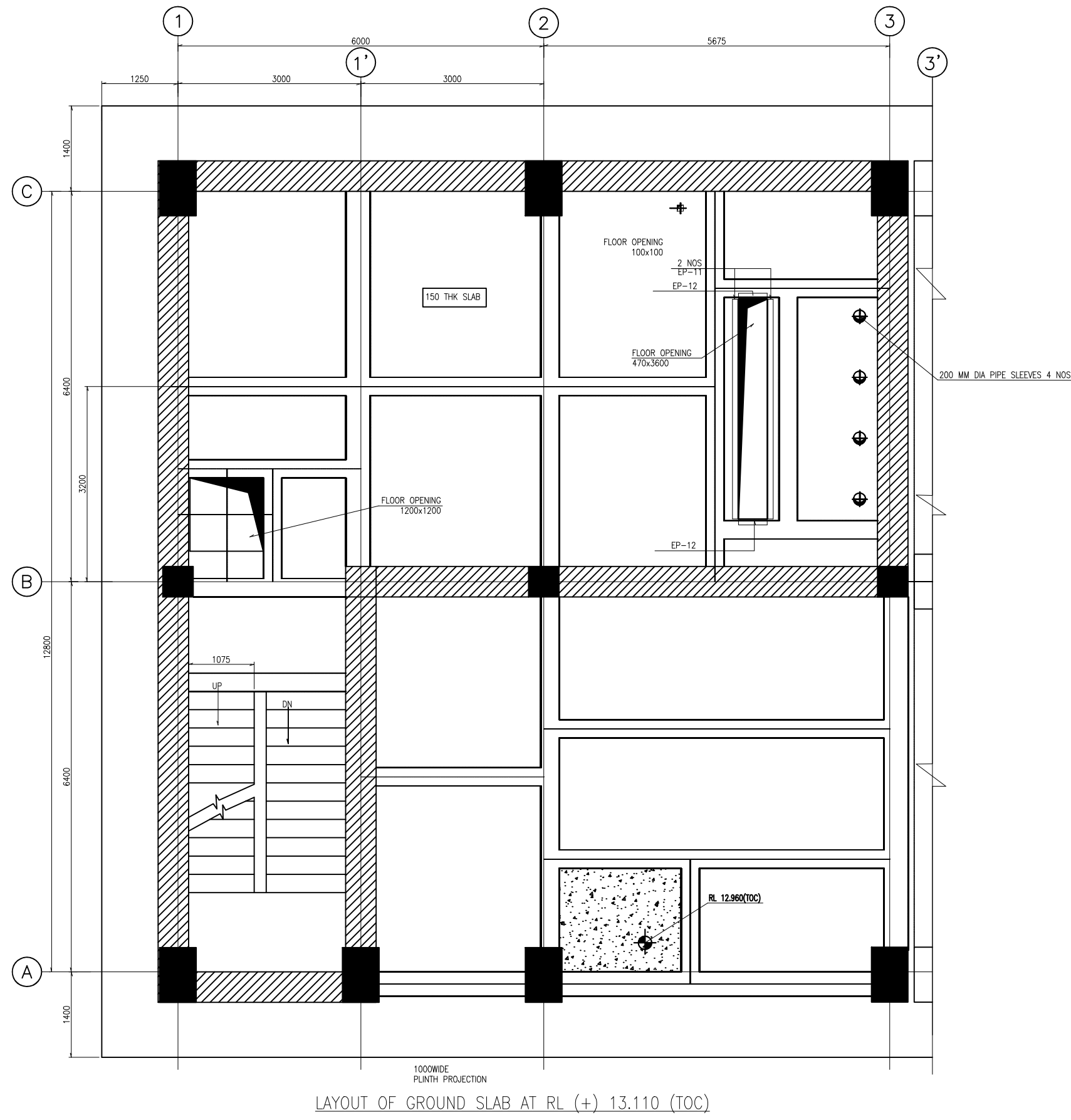
LAYOUT OF GROUND SLAB AT RL (+) 13.110 (TOC)
