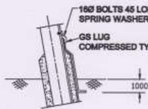
LUG FITTING (TYPICAL) FOR THREE LEGS
