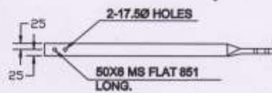
DETAILS OF FLAT TYPE 'C'
