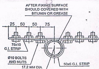
DETAIL-A for Cu-Bonded earth rod (For Pipe electrode it may be different)
